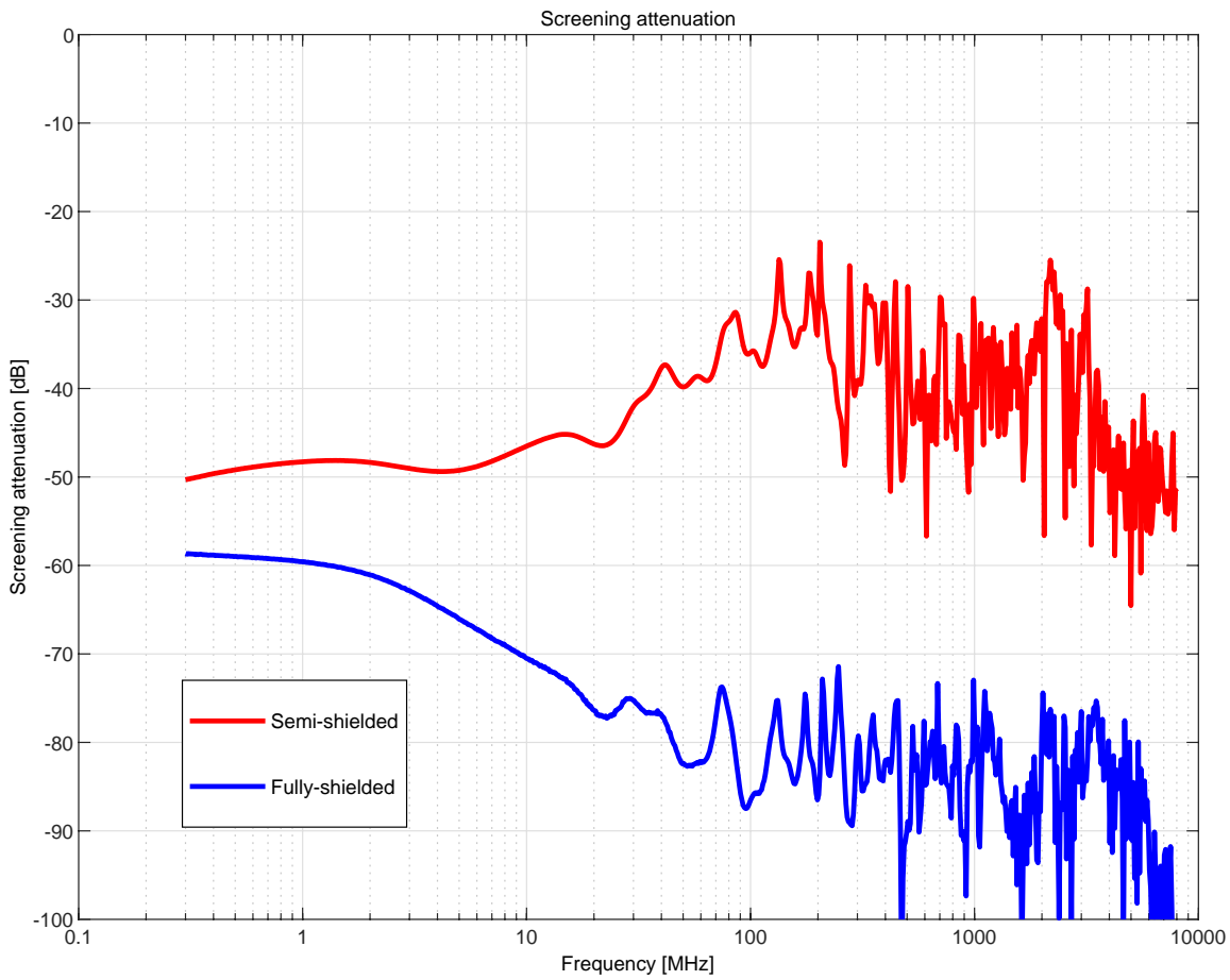
Figure 27: Screening attenuation
